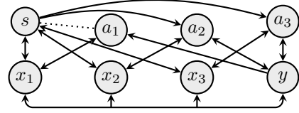
Figure 3: Orientation of non-explicit conflicts matters.
