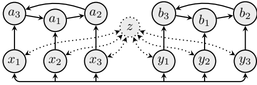
Figure 1: AFs illustrating the relations between various semantics.
